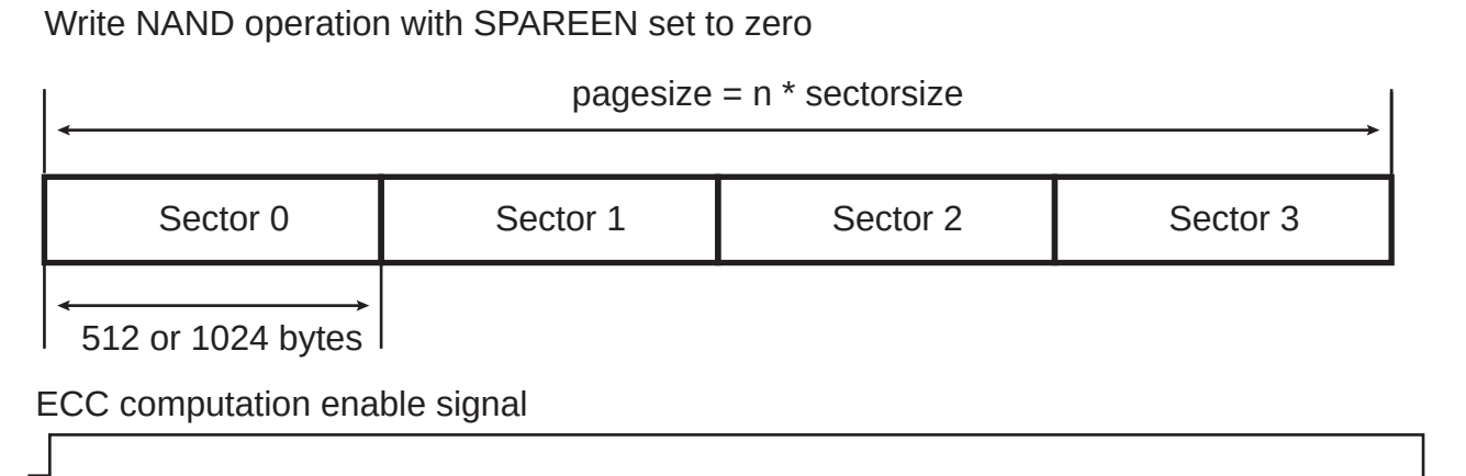
Figure 30-41.NAND Write Operation
