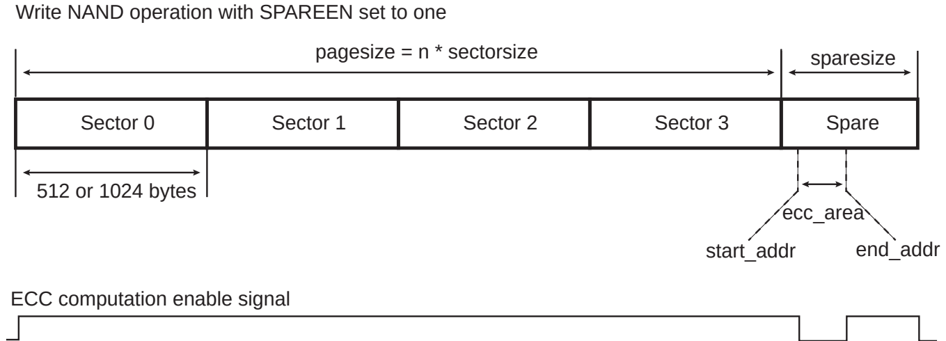
Figure 30-40.NAND Write Operation with Spare Encoding
